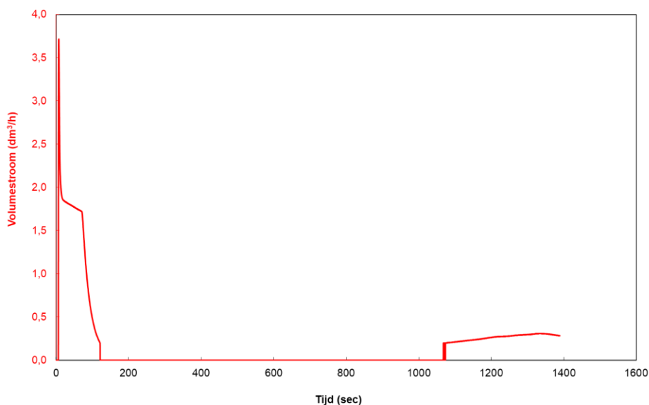
Figure 10 Typical measurement of air flow during the experiments, in this case of PVC 2016-064
